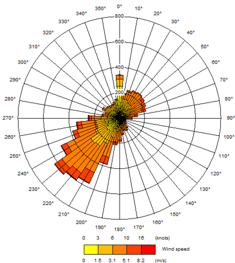
Figure 3.3 Wind Rose – Charlwood, 2022
